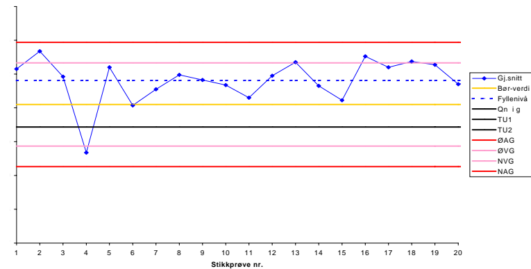
X-bar chart, n = 4
